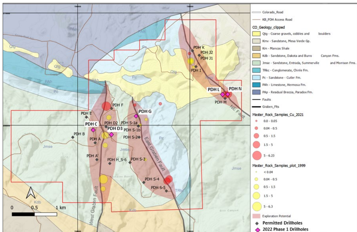
Figure 1. Klondike Geology and Copper Results Map
